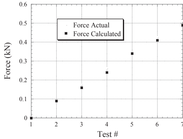
Figure 4.16 Results from loading the assembled and instrumented test apparatus used to calculate expected loading with a maximum 10% error.
