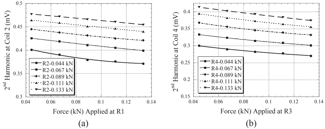
(a) (b) Figure 6.6 A decreasing sensor response was observed while monitoring from (a) coil 2 and (b) coil 4 with a changing load applied to R1 and R3 and constant loading applied to R2 and R4.
