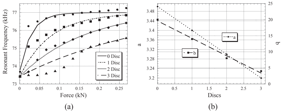
Figure 4.12 The (a) results and (b) coefficients of the applied decaying exponential curve fits from load testing of a 30.5 mm × 4.0 mm sensing strip from 0 N to 266 N at 22.2 N intervals with the distance between the applicator head and sensing strip adjusted from 0.0 μm to 40.0 μm at 20 μm intervals with an initial gap of 20 μm when no insert was placed underneath the support pillars of the applicator.
